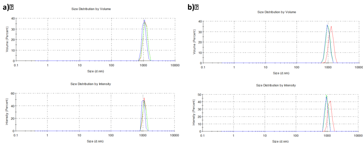
Figure S12. DLS data for DBS-CONH 2 H 2 /alginate two-component microgels prepared by mixing at 1000 (a) and 650 rpm (b).
