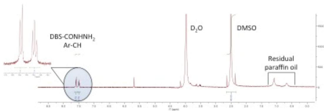
Figure S4. ^1\text{H} NMR of DBS-CONH \text{H}_2 /alginate microgel beads (100 \mu\text{L} aliquot of the original sample) after 20 mins at 90°C.
