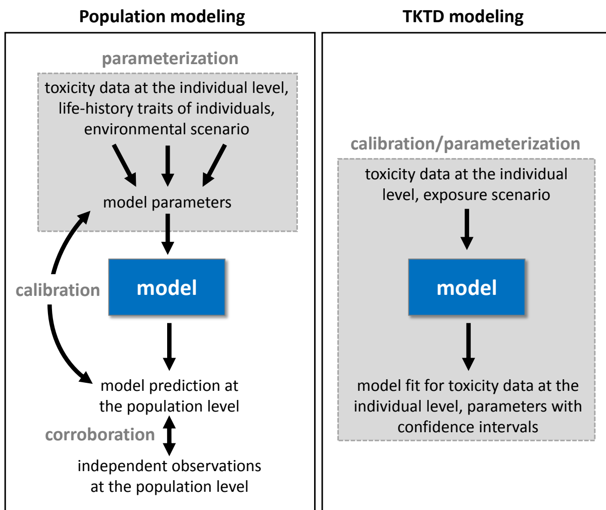
Figure 4. Difference between the typical use of population models and TKTD models. The grey box shows what ‘parameterisation’ involves for both types of models.
